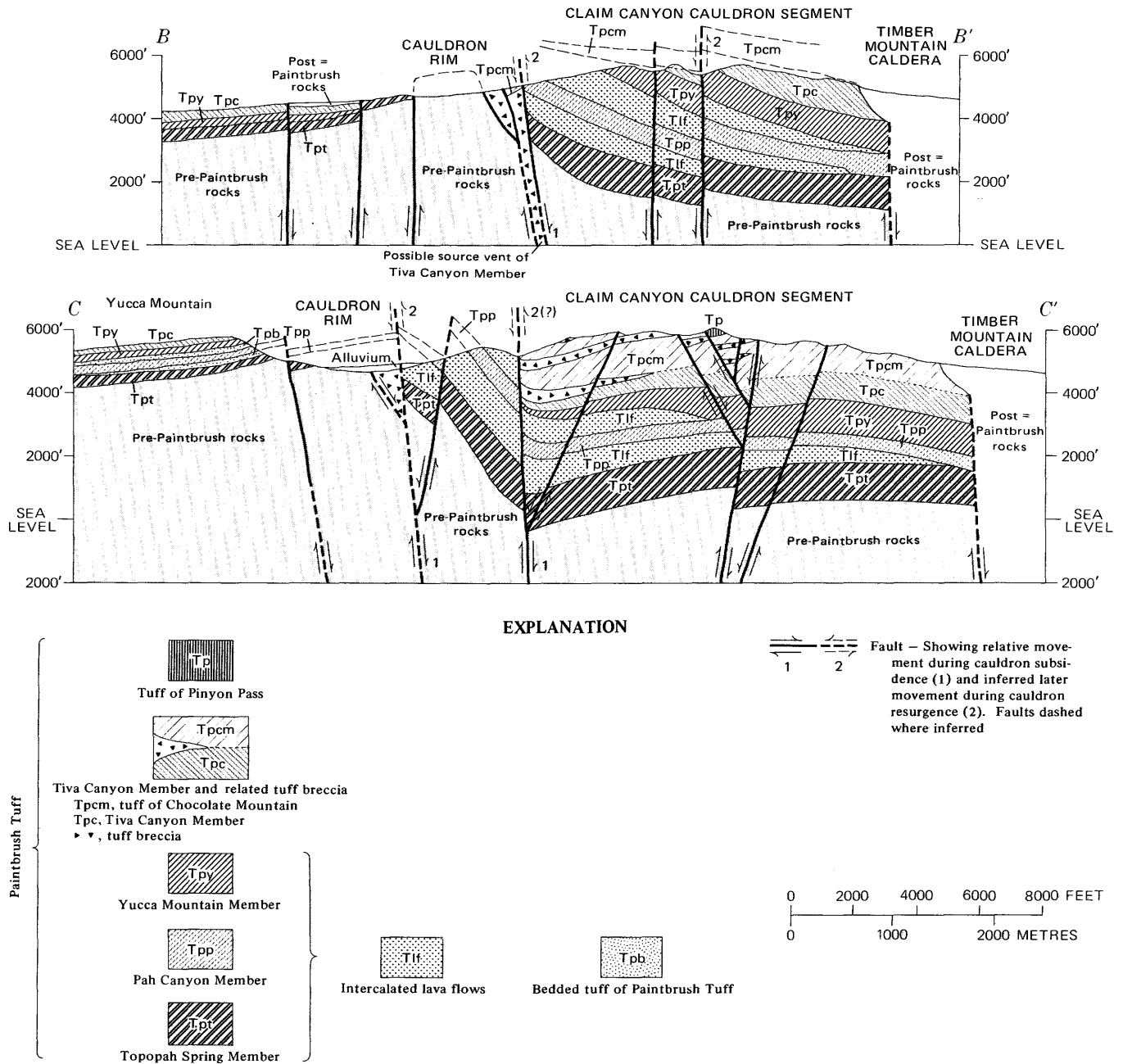
FIGURE 13.—Geologic sections through Claim Canyon cauldron segment, with critical units and faults projected above ground surface to indicate possible cauldron resurgence. Lines of sections shown in figure 12. Only major faults shown.
