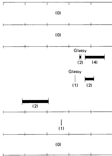
Peralkaline sequence of soda rhyolite lava, Grouse Canyon Member of Belted Range Tuff, and tuffs and lava and tuff of Deadhorse Flat (Noble, Sargent, and others, 1968, Orkild and others, 1968, 1969)
