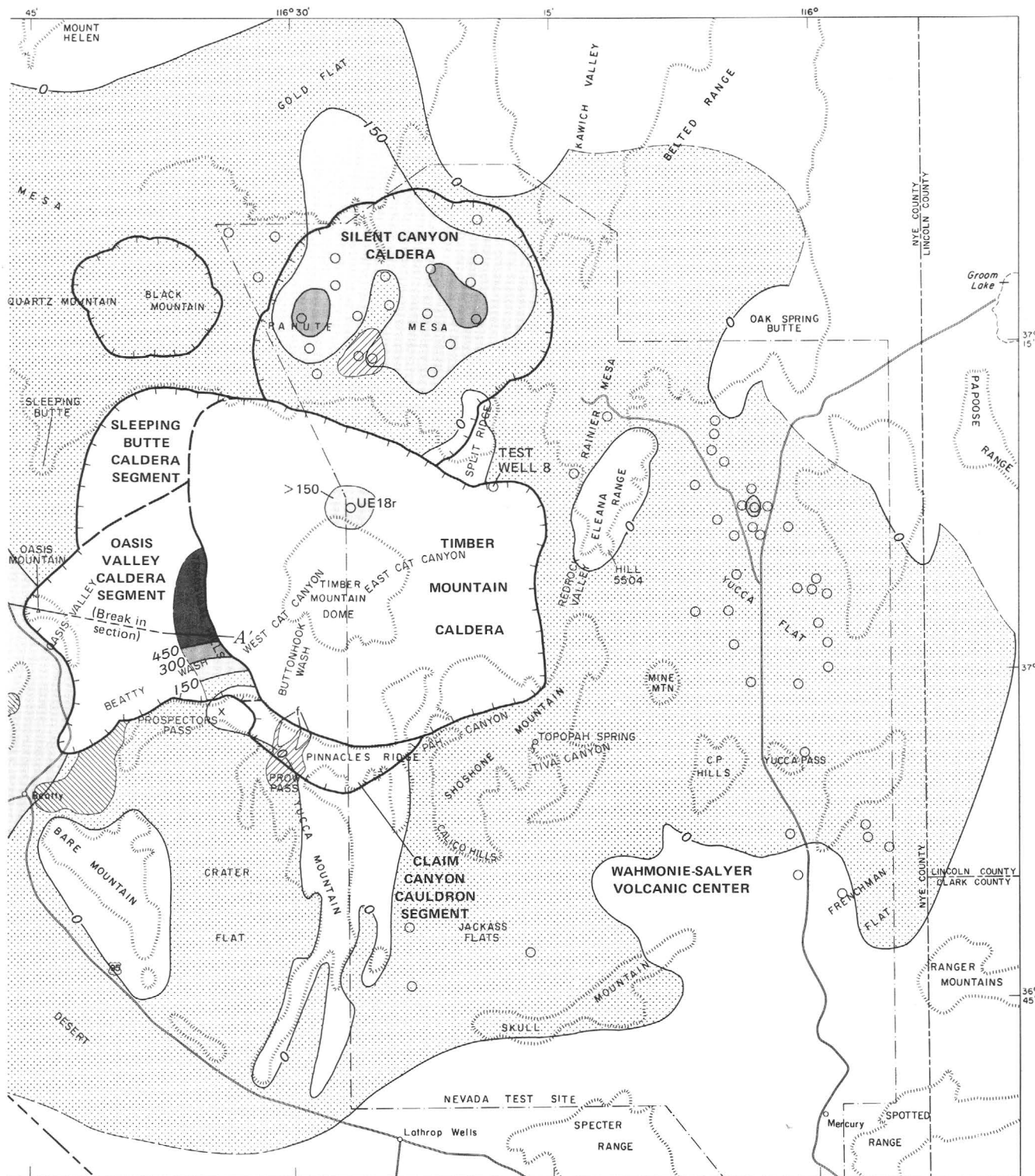
distribution of petrologically related, pre-Rainier Mesa lavas. Geologic cross section shown in figure 23.
