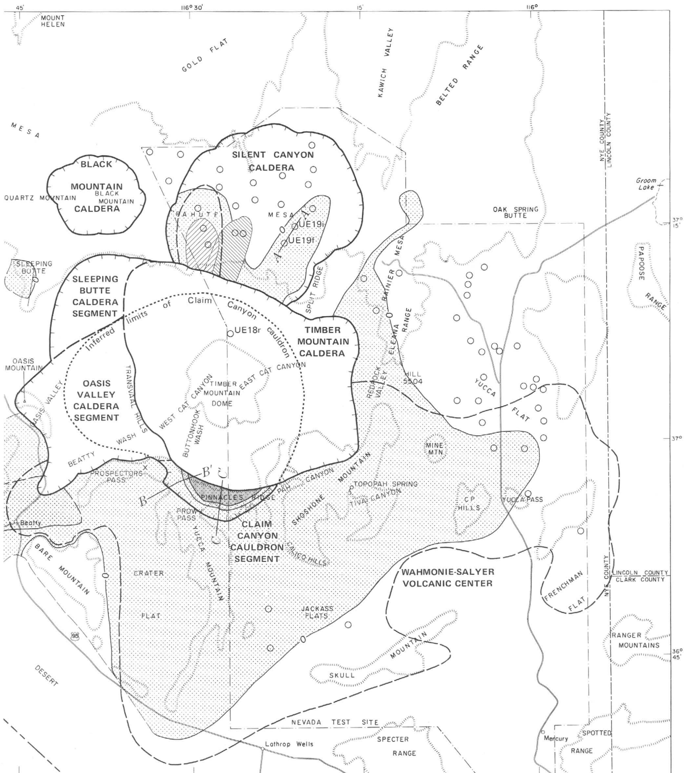
Member show great thickness of its uppermost subunit (tuff of Chocolate Mountain) within Claim Canyon cauldron segment. Geologic in figures 11, 12, and 13.
