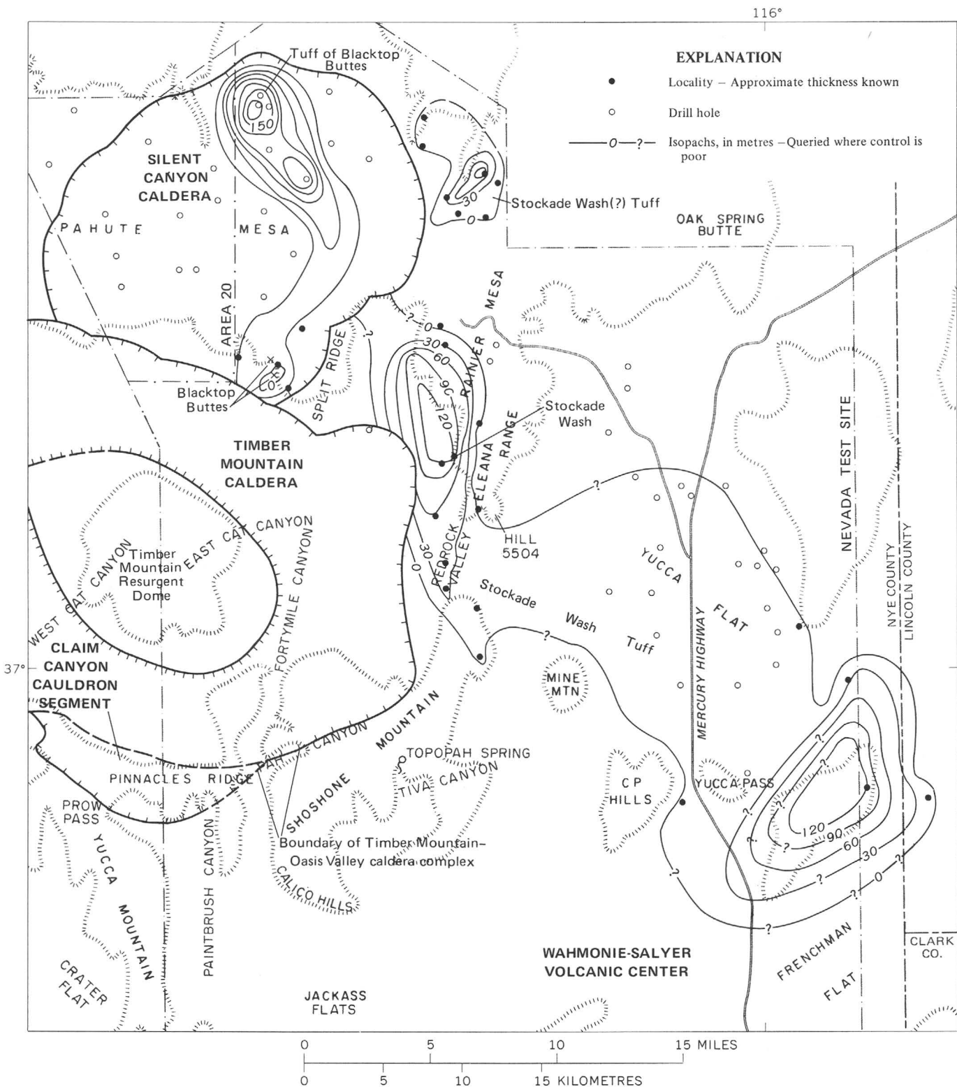
FIGURE 6.—Isopachs of Stockade Wash Tuff, Stockade Wash(?) Tuff, and tuff of Blacktop Buttes in relation to Silent Canyon caldera.
