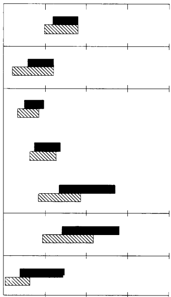
Peralkaline sequence of soda rhyolite lava, Grouse Canyon Member of Belted Range Tuff, and tuffs and lava and tuff of Deadhorse Flat (Noble, Sargent, and others, 1968, Orkild and others, 1968, 1969)
