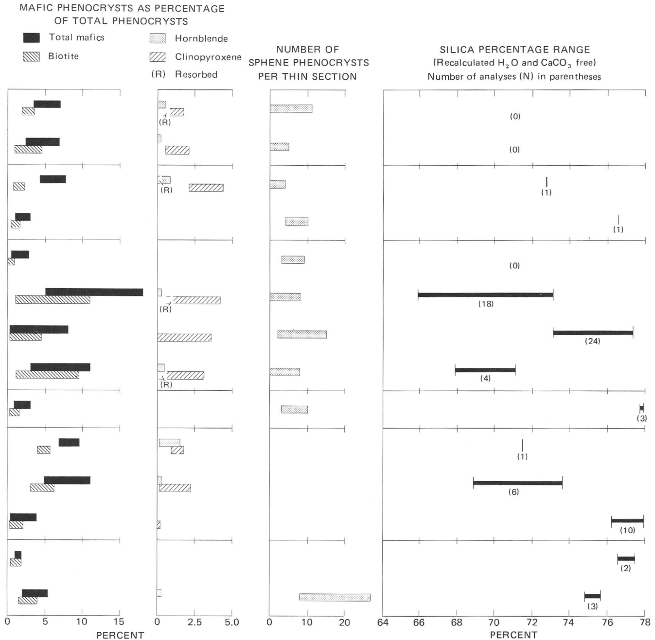
Modal analyses by F. M. Byers, W. D. Quinlivan, and J. T. O'Connor, and from Cornwall (1962, table 2). Silica percentages from Cornwall and P. W. Lipman (written commun., 1974).
