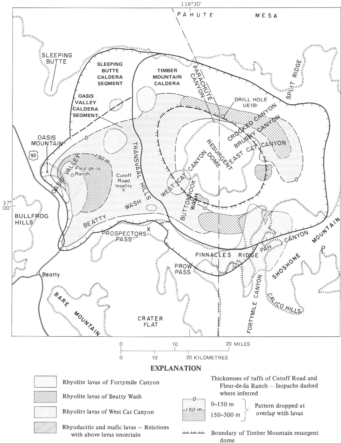
FIGURE 24.—Distribution of younger intracaldera rocks of Timber Mountain-Oasis Valley caldera complex. Rhyolite lavas of Beatty Wash in northern moat are inferred from drill-hole data and negative aeromagnetic anomaly.
