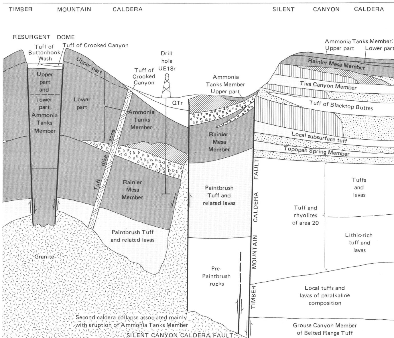
FIGURE 3 (left and above).—Generalized schematic diagram through southwestern Nevada volcanic field, showing geologic relations between ash-flow tuff sheets and related rocks discussed in this report. A few minor units omitted. Length of diagram about 50 km (30 mi).
