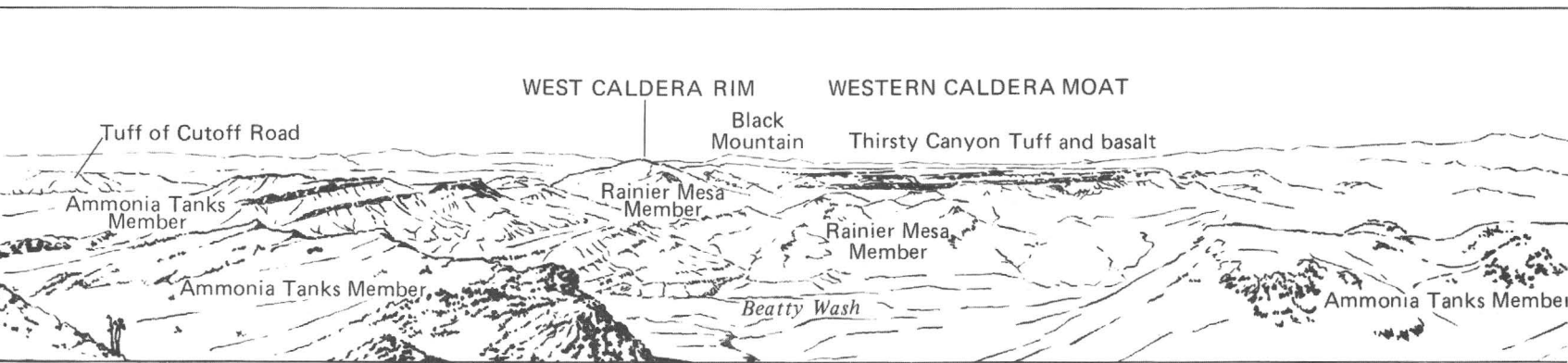
Panoramic view of Timber Mountain caldera from point southwest of Beatty Wash. Photograph by P. W. Lipman, 1964.
