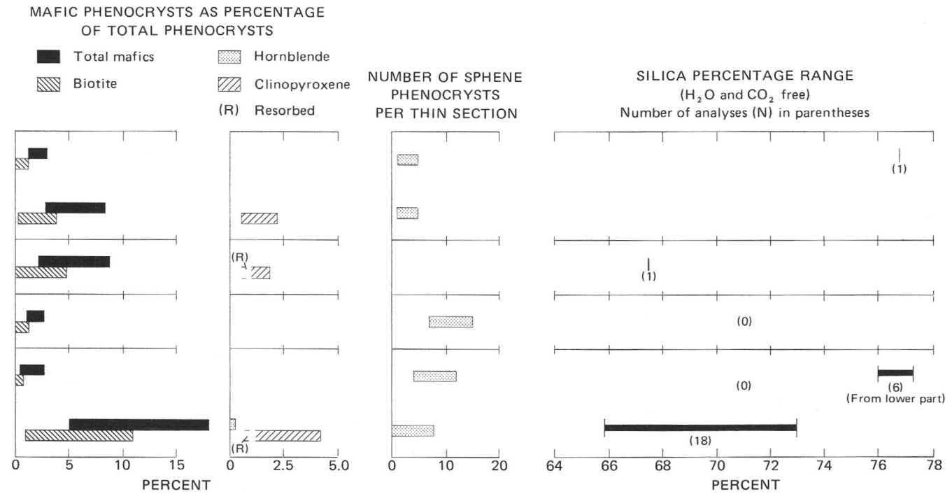
subunits of upper part of Ammonia Tanks Member. Age relations uncertain except that intrusive rocks generally postdate Ammonia Tanks W. D. Quinlivan and P. W. Lipman (written commun., 1974).
