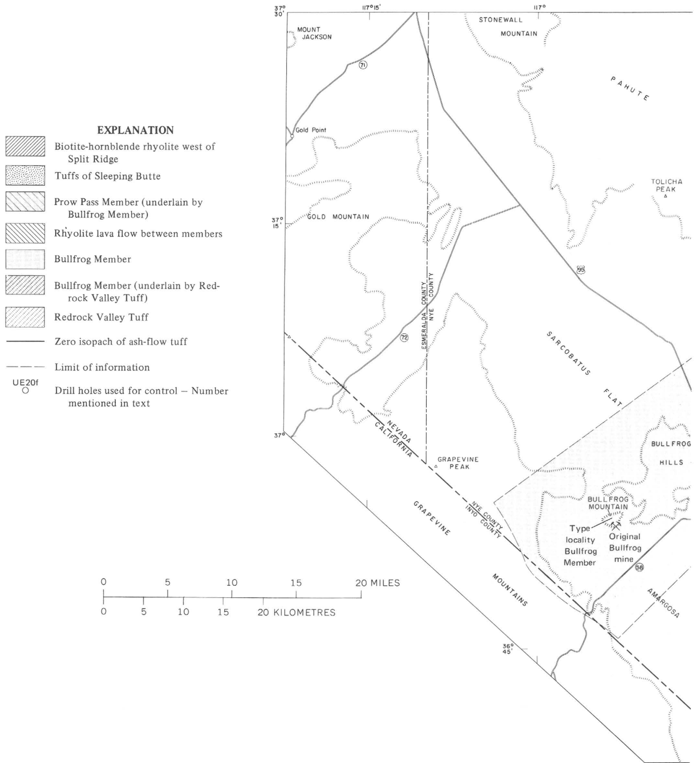
FIGURE 4.—Areal distribution of Redrock Valley Tuff, members of Crater Flat
