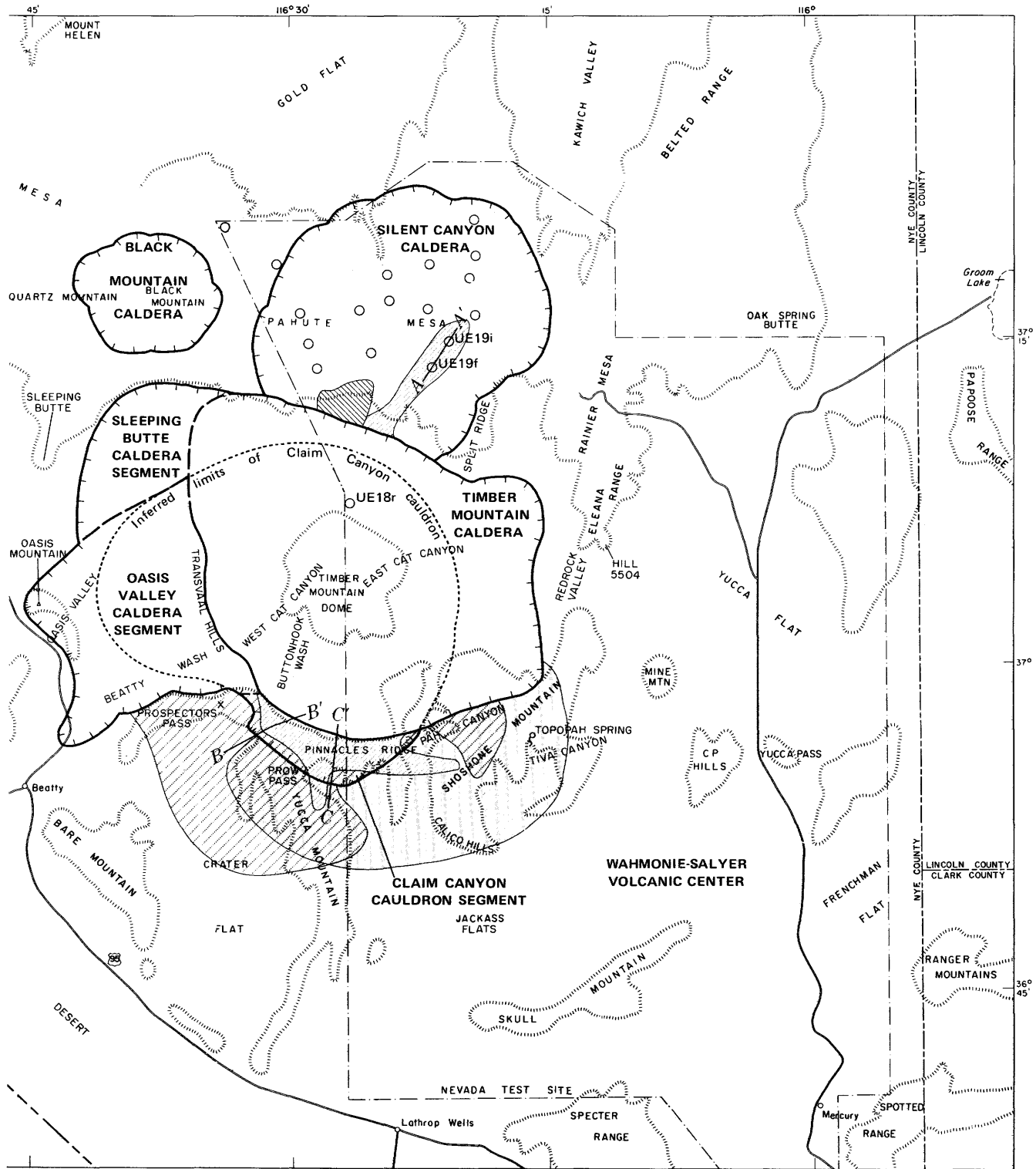
and extent of lavas between the members. Geologic cross sections shown in figures 11, 12, and 13.
