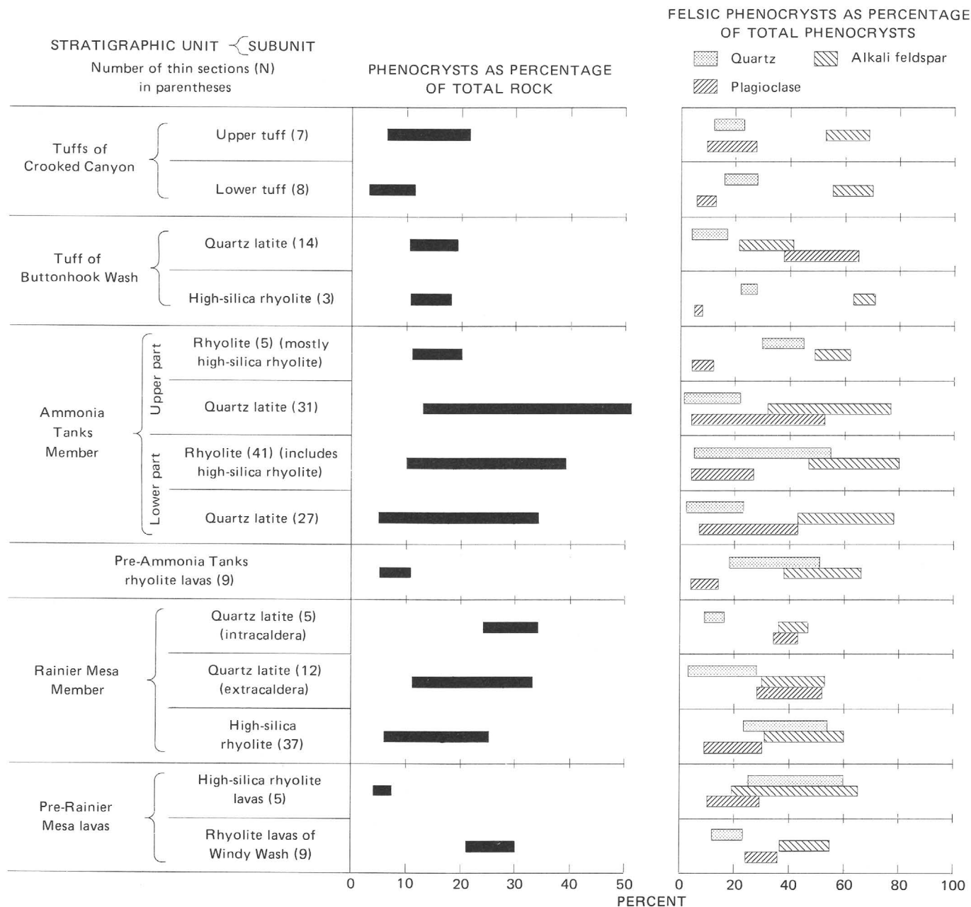
FIGURE 15.—Modal and silica ranges of units of Timber Mountain Tuff and petrologically related lavas in order of stratigraphic succession. (1962), Lipman (1966), and W. D. Quinlivan
