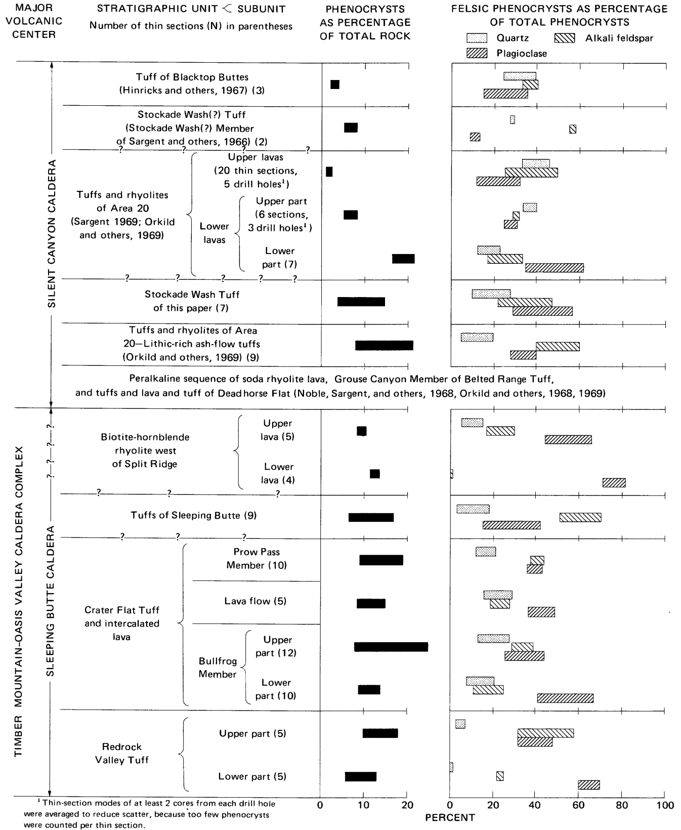
FIGURE 5.—Modal and silica ranges of Redrock Valley, Crater Flat, and Stockade Wash Tuffs and petrologically related lavas in general
