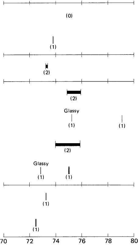
Peralkaline sequence of soda rhyolite lava, Grouse Canyon Member of Belted Range Tuff, and tuffs and lava and tuff of Deadhorse Flat (Noble, Sargent, and others, 1968, Orkild and others, 1968, 1969)
