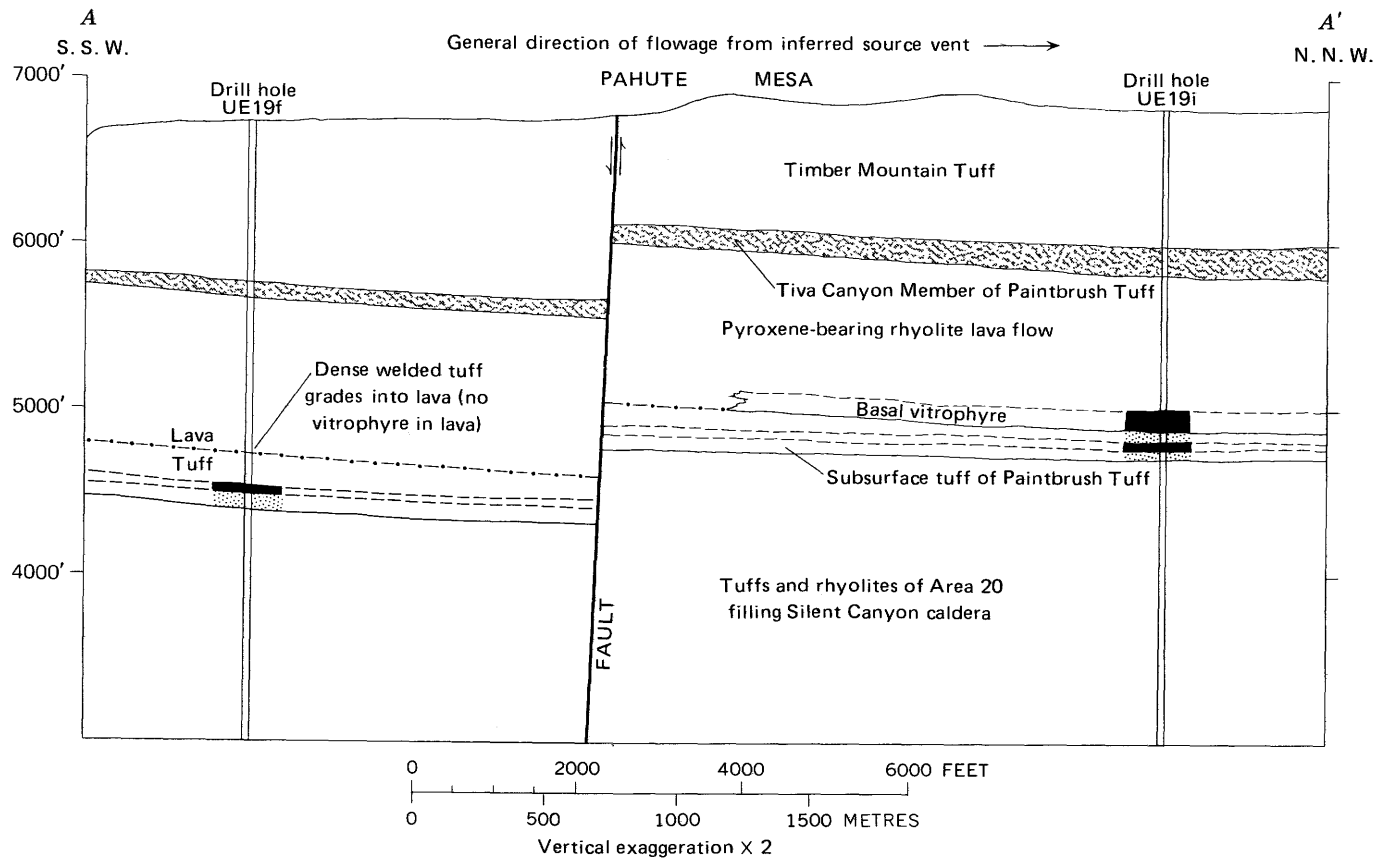
FIGURE 11.—Generalized section along A-A' through drill holes UE19f and UE19i, Silent Canyon caldera, showing relations between subsurface ash-flow tuff of Paintbrush Tuff and overlying, mineralogically similar pre-Tiva Canyon rhyolite lava. Vitrophyres shown in black; nonwelded to partially welded zones, stippled. Inferred transitional contact shown by dot-dash line. Line of section shown in figures 8, 10.
