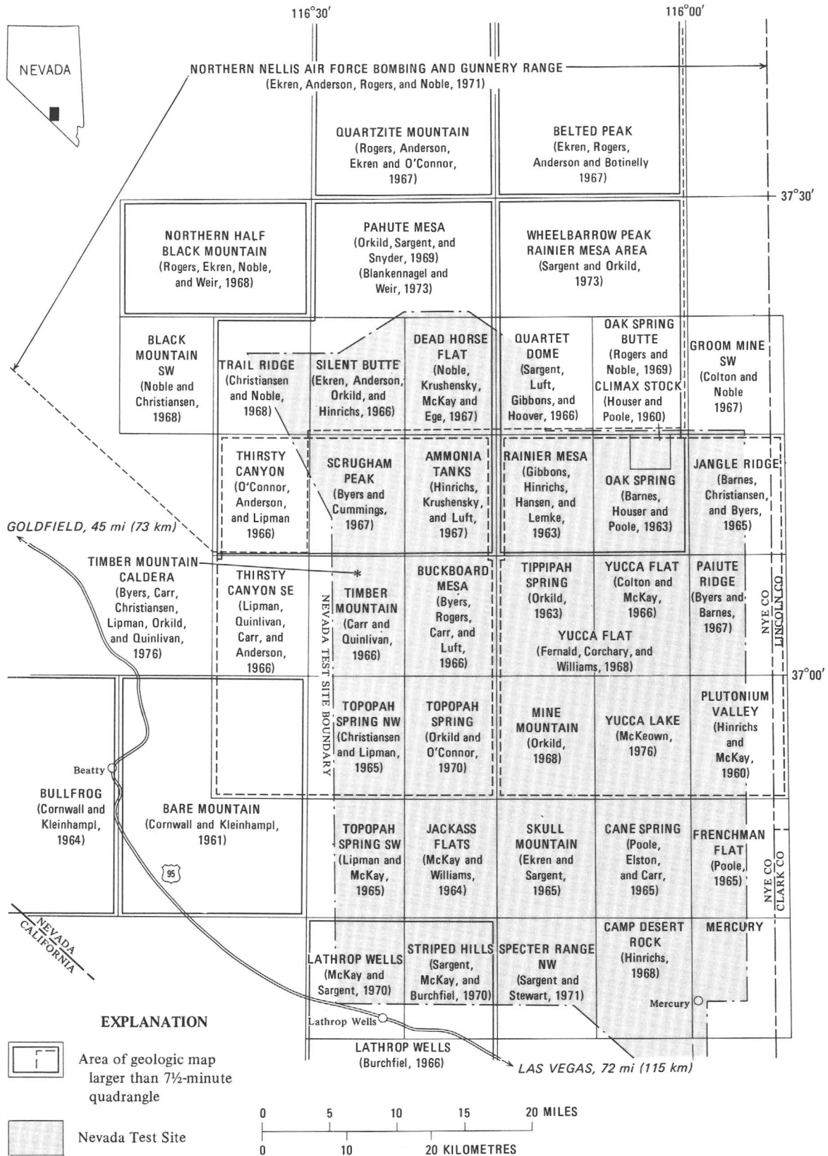
FIGURE 2.—Index showing original sources of geologic data and other maps published by the U.S. Geological Survey for the Timber Mountain caldera area, Nevada Test Site, and adjacent region. Mapped areas are identified by author and date and are listed in the references at the end of the text.
