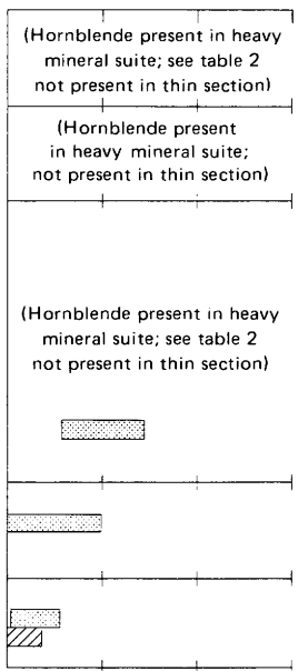
Peralkaline sequence of soda rhyolite lava, Grouse Canyon Member of Belted Range Tuff, and tuffs and lava and tuff of Deadhorse Flat (Noble, Sargent, and others, 1968, Orkild and others, 1968, 1969)
