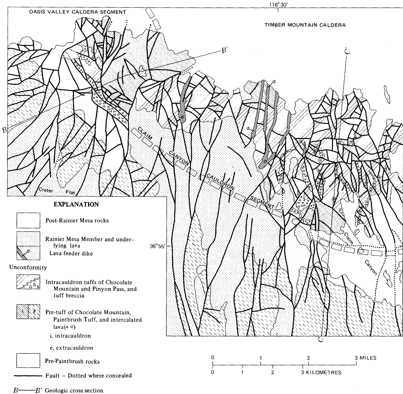
FIGURE 12.—Generalized geologic map of Claim Canyon cauldron segment and vicinity, showing greater intensity of faulting of tuffs within cauldron than outside. Generalized from geologic map of Timber Mountain caldera (Byers and others, 1976).
