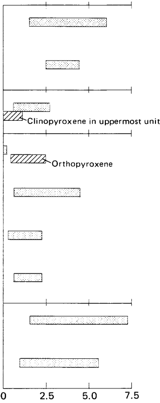
Peralkaline sequence of soda rhyolite lava, Grouse Canyon Member of Belted Range Tuff, and tuffs and lava and tuff of Deadhorse Flat (Noble, Sargent, and others, 1968, Orkild and others, 1968, 1969)
