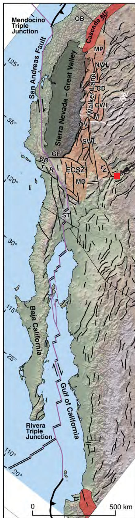
Figure 12. Present-day configuration of the Pacific – North American plate boundary including the short spreading centers and long, right-stepping dextral transform segments in the Gulf of California (Rivera triple junction to the Salton Trough [ST]); the relatively narrow San Andreas transform fault system (Salton Trough to the Mendocino triple junction with the left-jogging, transpressional “big bend” in southern California); and the broader Walker Lane – eastern California shear zone, which splays from the San Andreas just east of the big bend and shunts some relative plate motion east of the Sierra Nevada block. Slate Ridge is south of the Big Bend and shows substantial trans-extensional tectonic motions, including rotation of adjacent blocks. The Walker Lane terminates northwestward near the south end of the Cascade arc (inboard of the Mendocino triple junction) and against the clockwise-rotating Oregon block.
